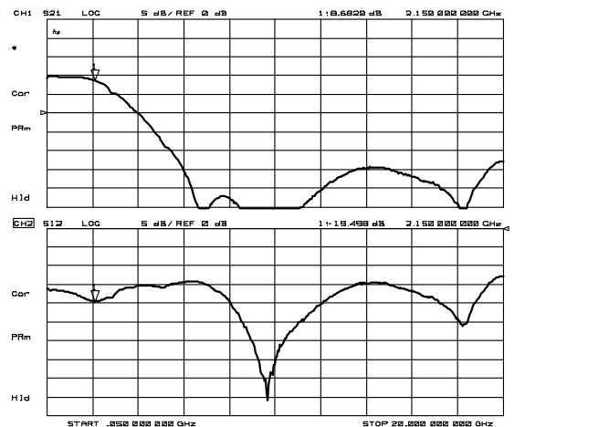
S21, S12 (f=50MHz~20GHz)
